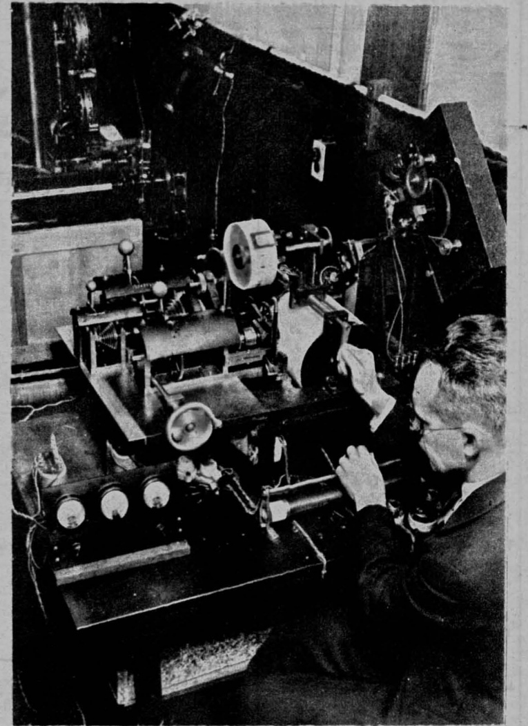
STUDIES STRUCTURE OF MATTER » Prof. G. R. Harrison, Massachusetts Institute of Technology (Boston), operates a machine designed to measure and compute the wave-lengths of spectrum lines. KEYSTONE PHOTO
